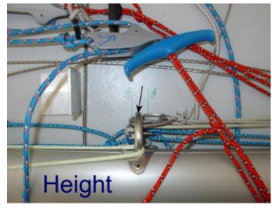
Rigging points: shroud, forestay, trapeze. Heights to be measured from MDP.
