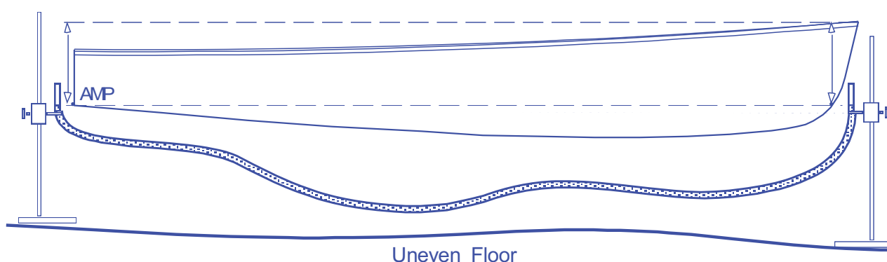
Figure F.6.5.3 A water tube for precisely levelling a hull on which baseline reference points have been established according to the class rules.
